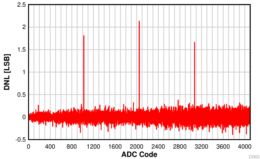
Figure 8-23. DNL vs. ADC Code
