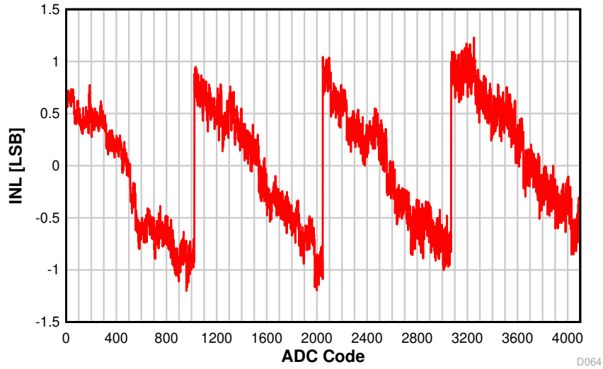
Figure 8-22. INL vs. ADC Code
